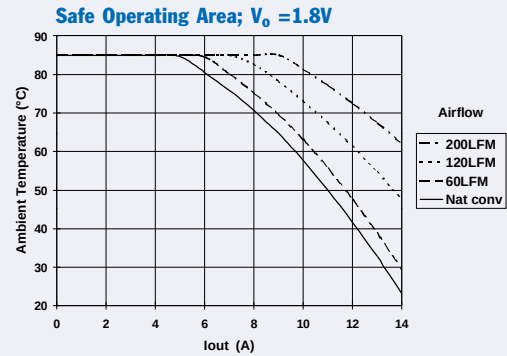
PT6722 Thermal Derating; V_{in} = 12V (See Note A)
