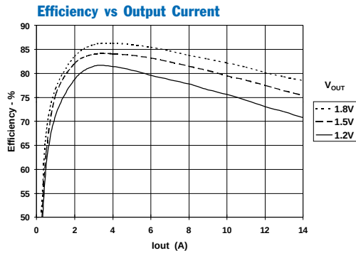
PT6722 Performance; V_{in} = 12V (See Note A)
